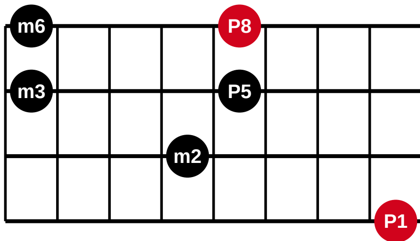
4 strings - 8 frets - fingering 6 of 10
